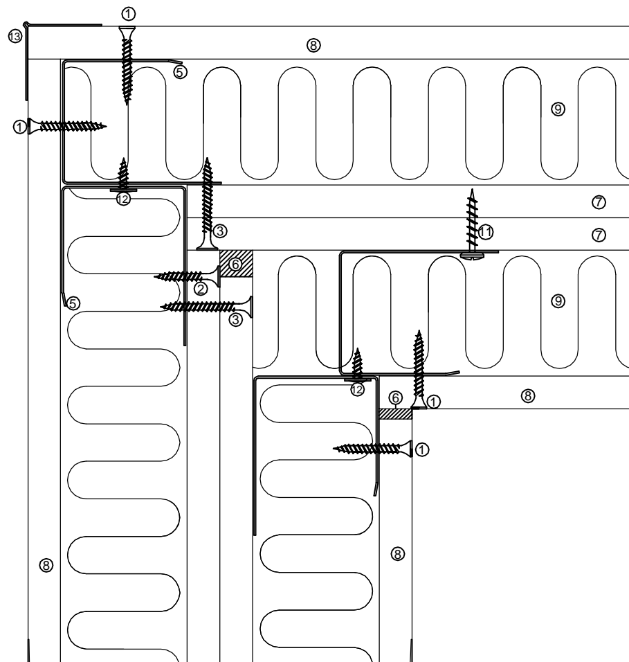
Detail F
