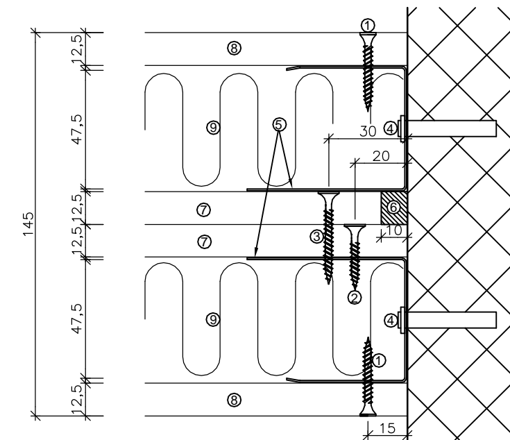
Detail D
